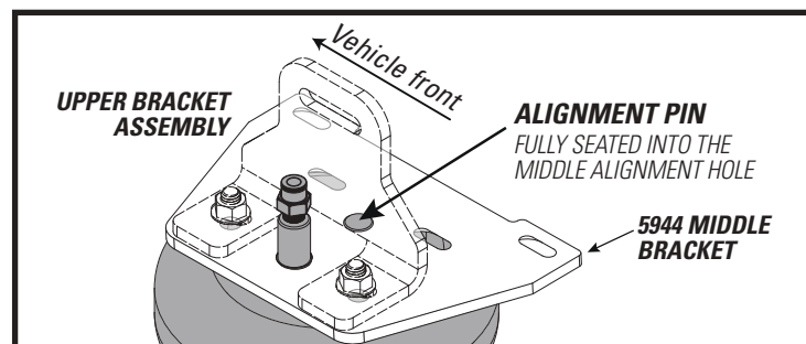
ALIGNMENT DETAIL
